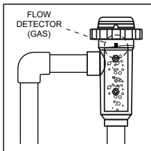
RECOMMENDED installation
