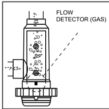
UNACCEPTABLE installation
